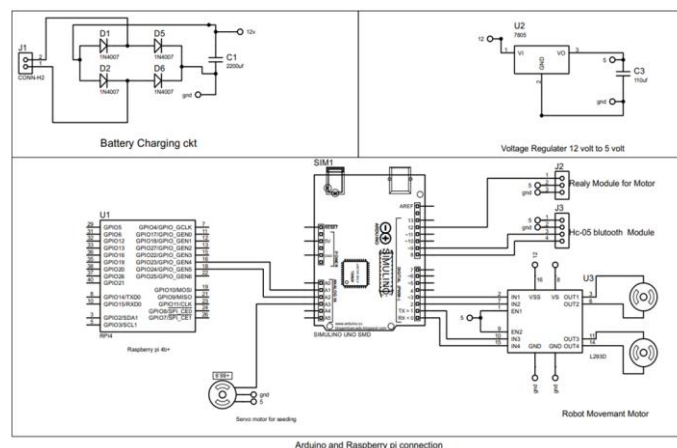
Figure 3. Circuit Diagram
