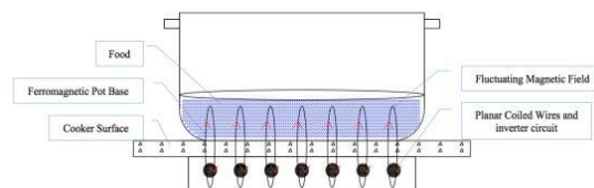
Figure 1. Induction cooker
