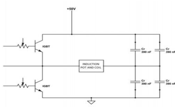
Figure 7. Half bridge circuits
